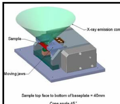
Tensile stages for X-ray diffractometer applications
