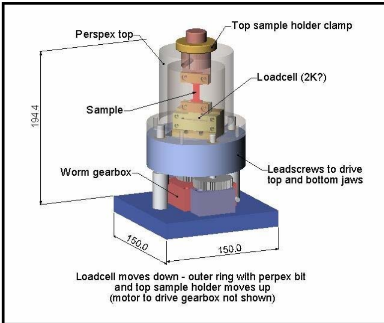
Tensile stage for X-Ray tomography applications
