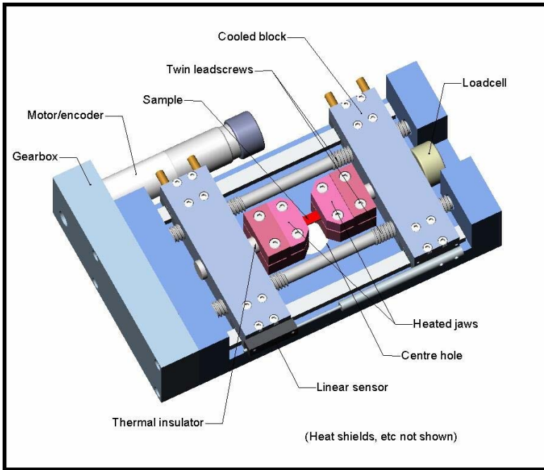
Tensile stage with heating for synchrotron applications
