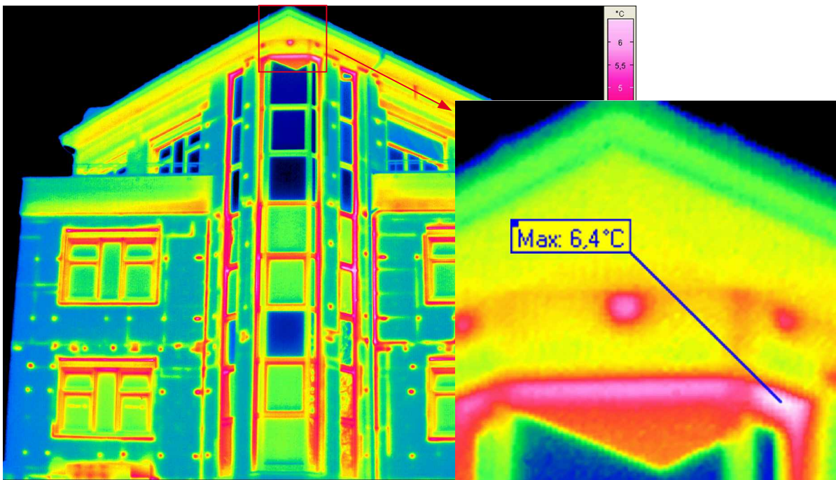
Img. 3: Resolution Enhancement mode of (640 x 480) pixel detector resulting in (1.280 x 960) = 1.228.infrared pixels
