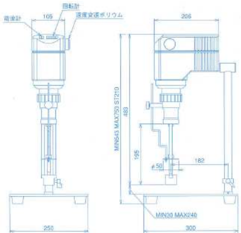
▲HOMOGENIZING MIXER MARK II 2.5型
