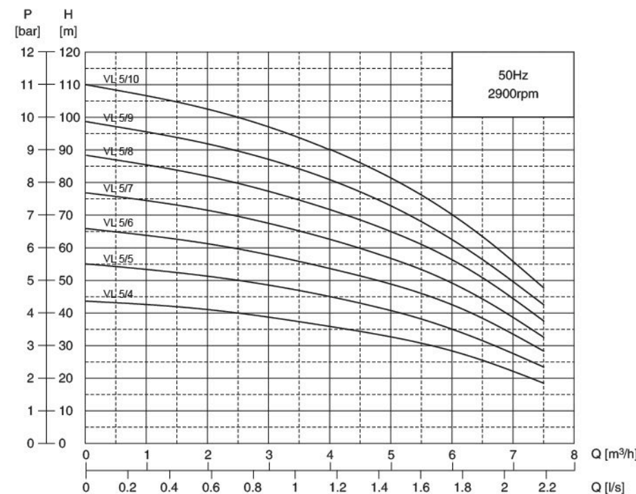
PERFORMANCE CURVE CHART 性能曲线图
