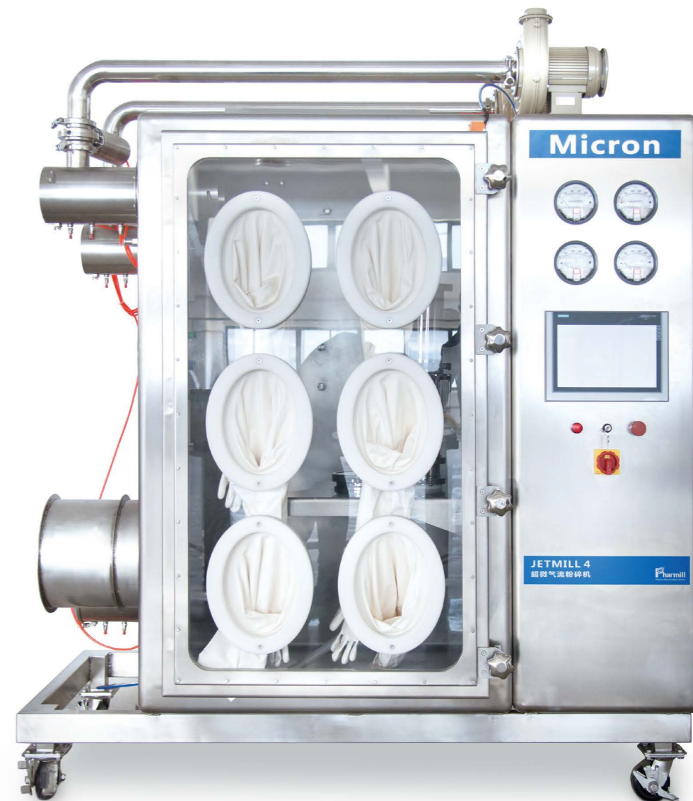
生产型密闭隔离粉碎 Commercial type isolating crusher
