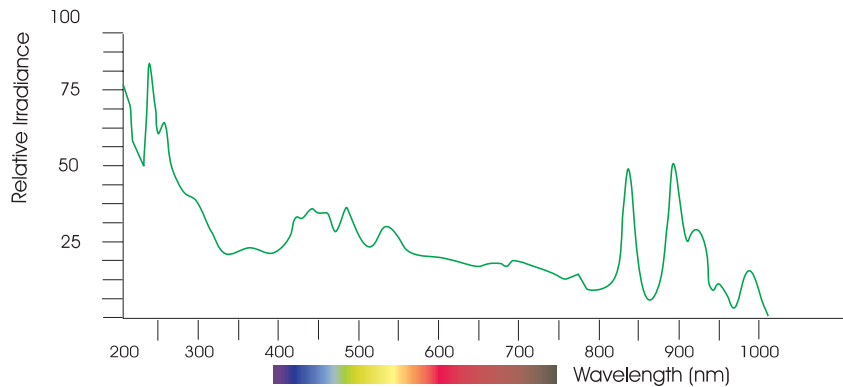
Spectral output of the AvaLight-XE-HP
