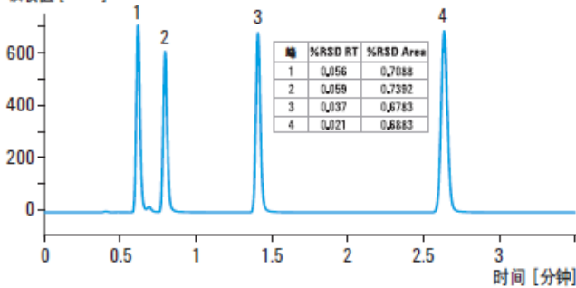
ZORBAX Eclipse Plus C18, 3.0 x 50 mm, 1.8 μm 吸收值 [mAU]
