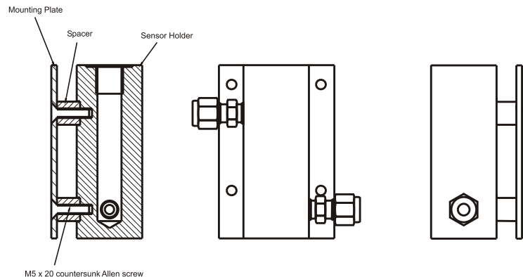
Shaw Sensor Holder. General Arrangement
