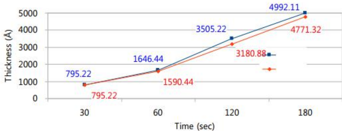
Time Vs Ashing thickness
