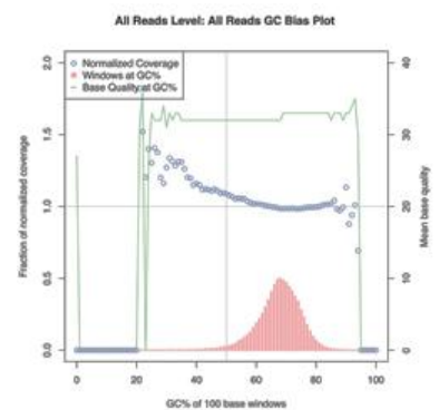
GC-rich
