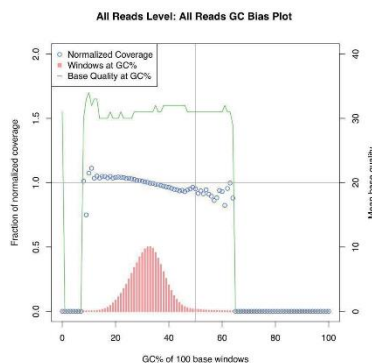
AT-rich
