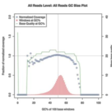
AT-GC even
