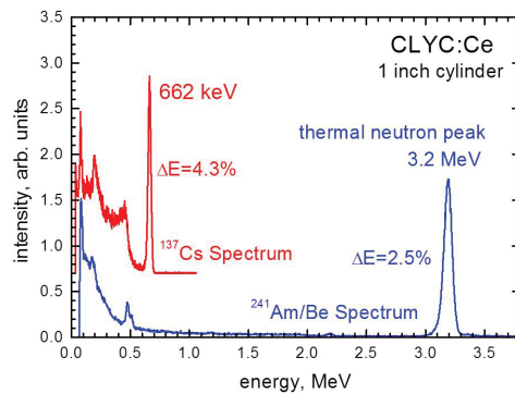
Gamma and Neutron Energy Spectra
