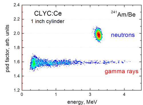
Pulse Shaped Discrimination
