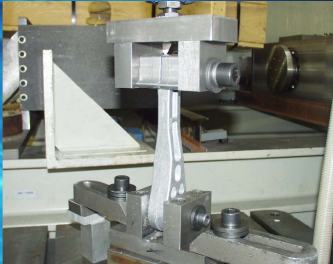
Test of Brackets
