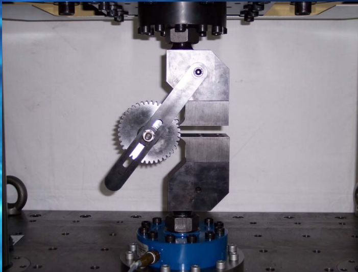
Gear Tests (Tooth Bending)
