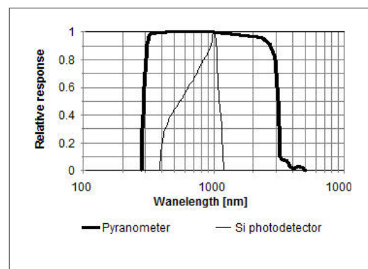
Fig. 1. PMA2145 Spectral Response vs Response of a Si photodiode
