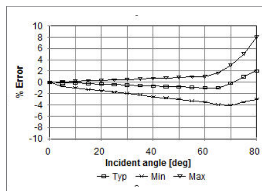
Fig. 2. PMA2145 Angular Response
