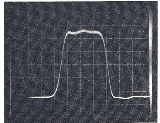
Detected Pulse Response (5 ns/div.)
