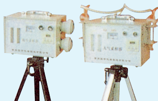
CD-2/BFC-35B 双流量大气/粉尘仪 CD-2/BFC-35B Double Air Current Atmosphere/Powder Dust Instrument
