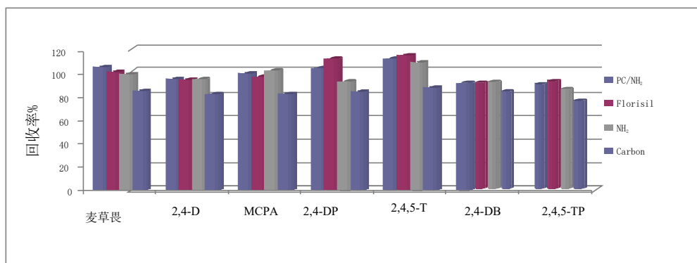
图43 4种固相萃取净化柱对农科院花园土壤提取液中7种苯氧羧酸类农药的吸附
