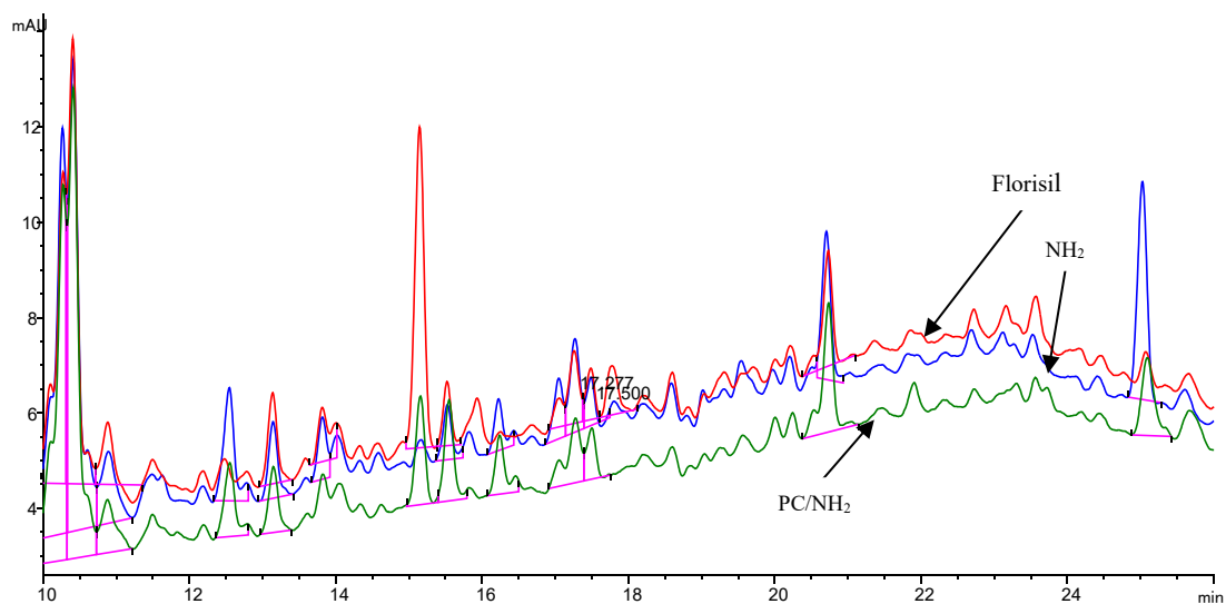
图41 4种固相萃取净化柱对崂山水库底泥提取液中7种苯氧羧酸类农药的吸附
