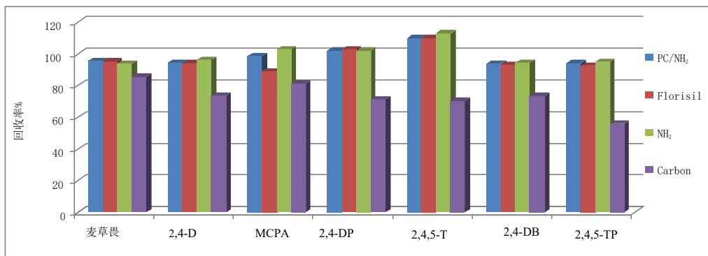
图41 4种固相萃取净化柱对崂山水库底泥提取液中7种苯氧羧酸类农药的吸附
